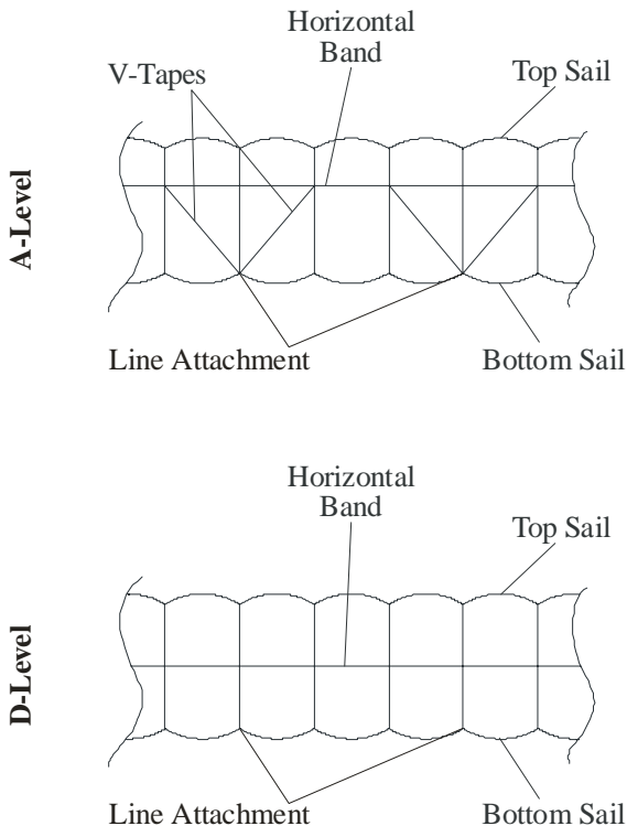
Illustration 1: Construction of the canopy with ribs and H-tapes
