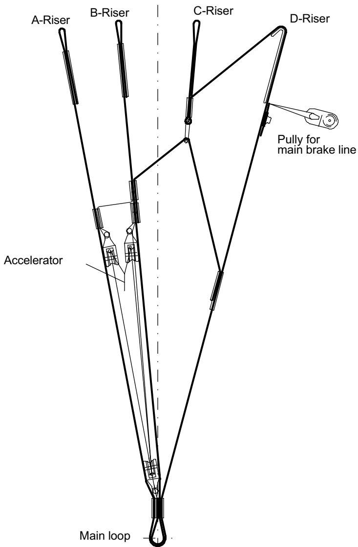
Illustration 2: UP Summit 2 Riser
