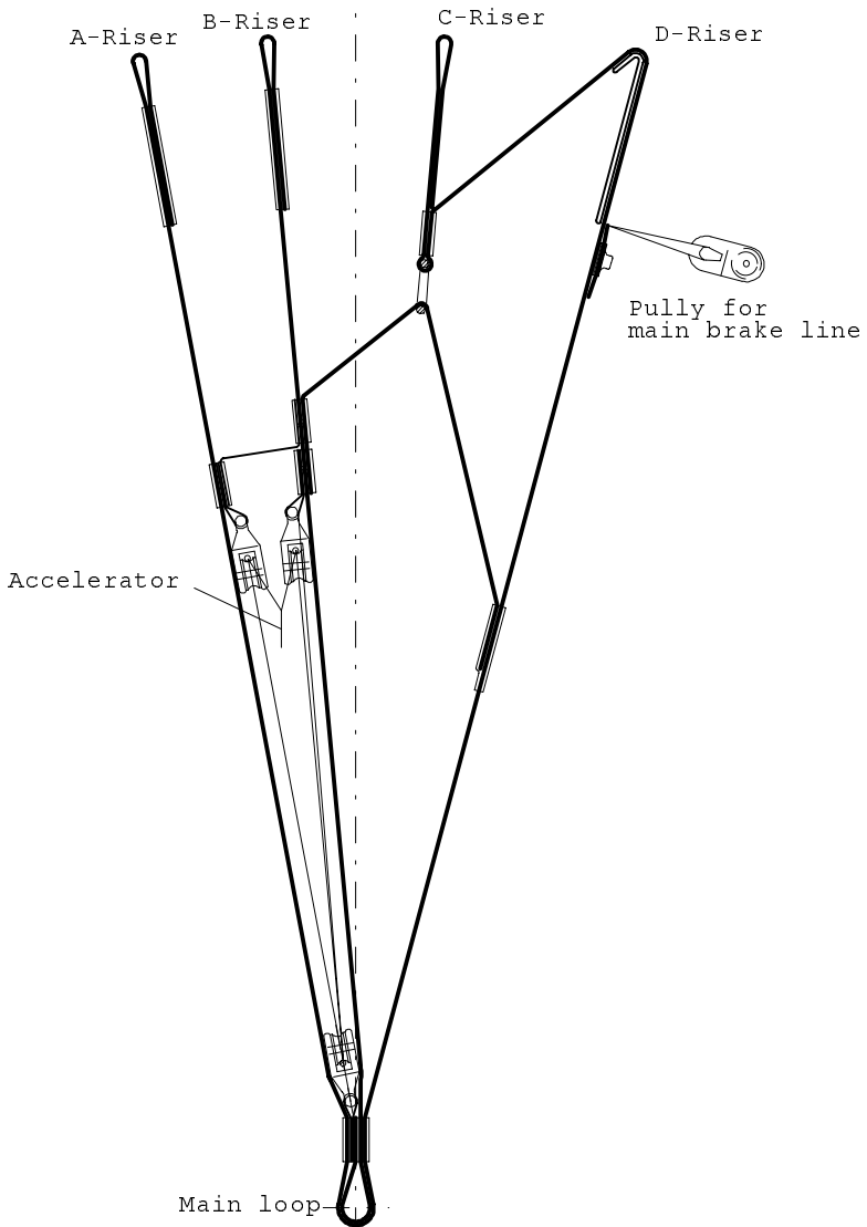
Illustration 2: UP Summit Riser
