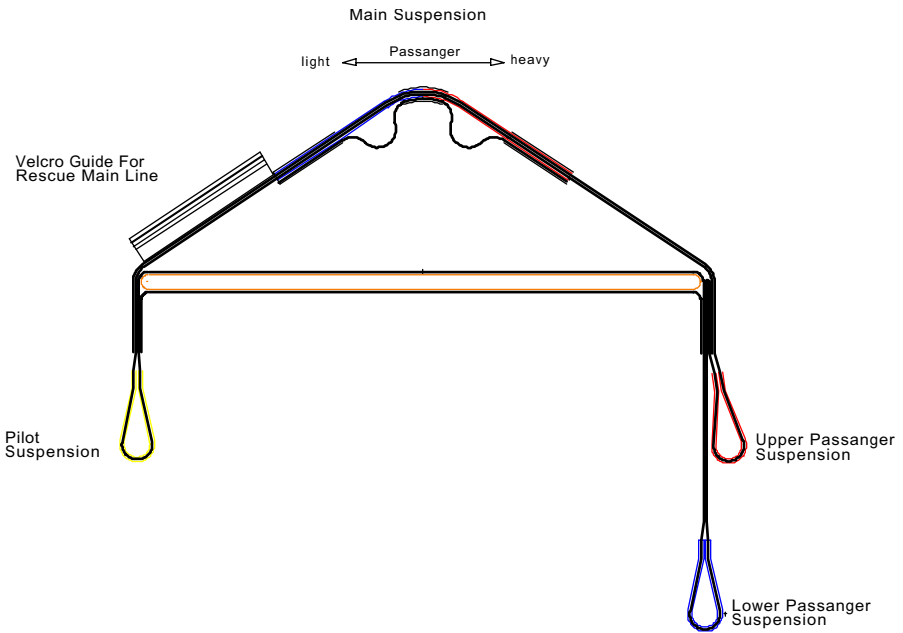
Illustration 2: UP Sherpa T-Bars
