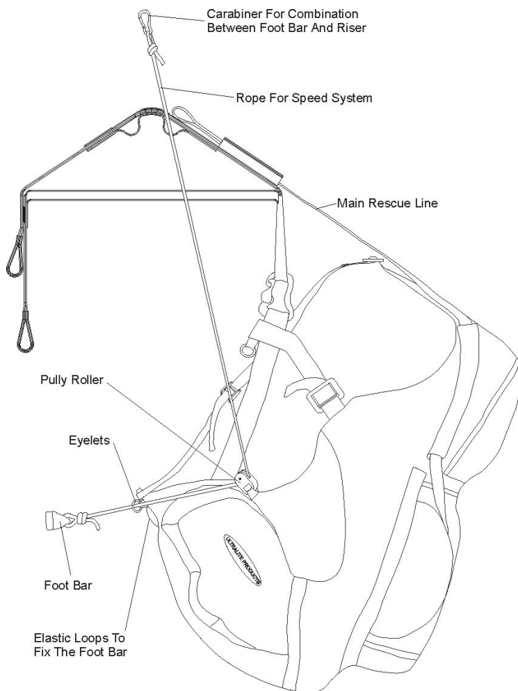
Illustration 7: Components of the foot accelerator and the rope course
