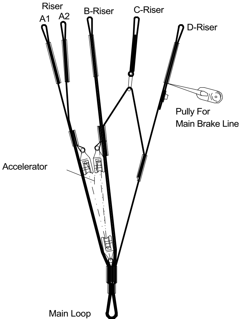
Illustration 1: UP Sherpa Riser
